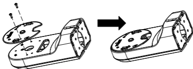
Figure 2-16 Install the Installation Plate
