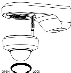
Figure 2-25 Secure DE2xxx Series PTZ Camera
