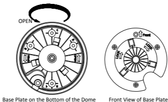
Figure 2-21 Base Plate for DE2xxx Series PTZ Camera
