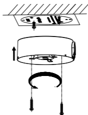
Figure 2-40 Fix the Junction Box
