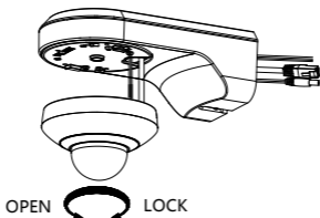
Figure 2-19 Install the Camera
