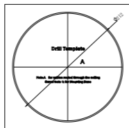
Figure 2-56 Drill Template
